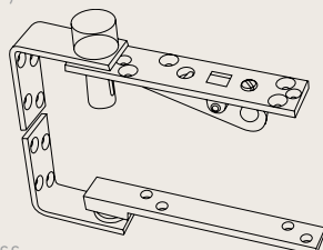
PS.110 - Pivot set with adjustable top centre, bottom strap and door frame fixing bracket (12mmØ)
